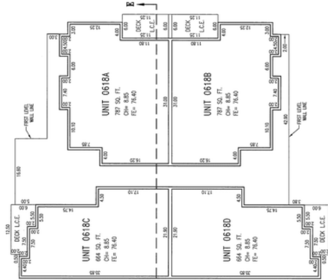
BUILDING 5 SECOND LEVEL INTERIOR WALLS 0.67' WIDE EXTERIOR WALLS 0.67' WIDE
