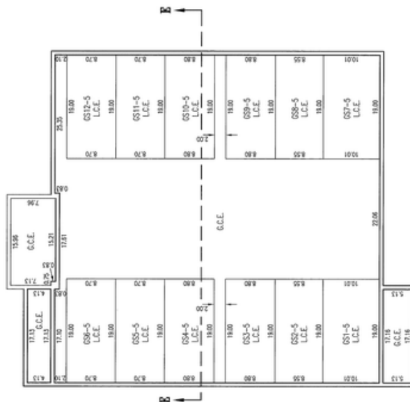
BUILDING 5 FIRST LEVEL INTERIOR WALLS 0.67' WIDE EXTERIOR WALLS 0.67' WIDE
