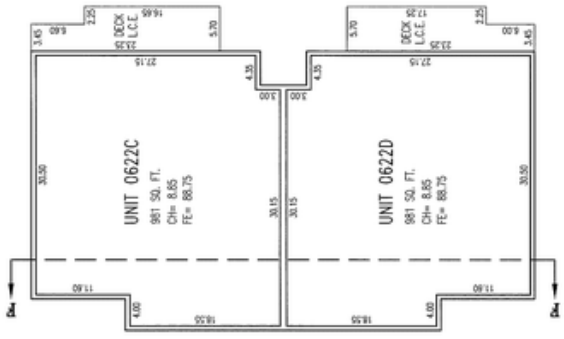
BUILDING 6 THIRD LEVEL INTERIOR WALLS 0.67" WIDE EXTERIOR WALLS 0.55" WIDE
