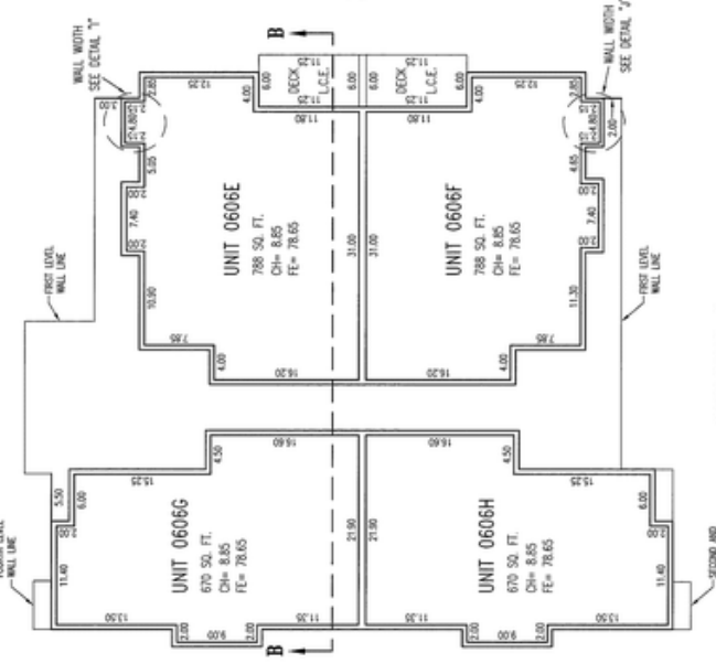
BUILDING 2 THIRD LEVEL
