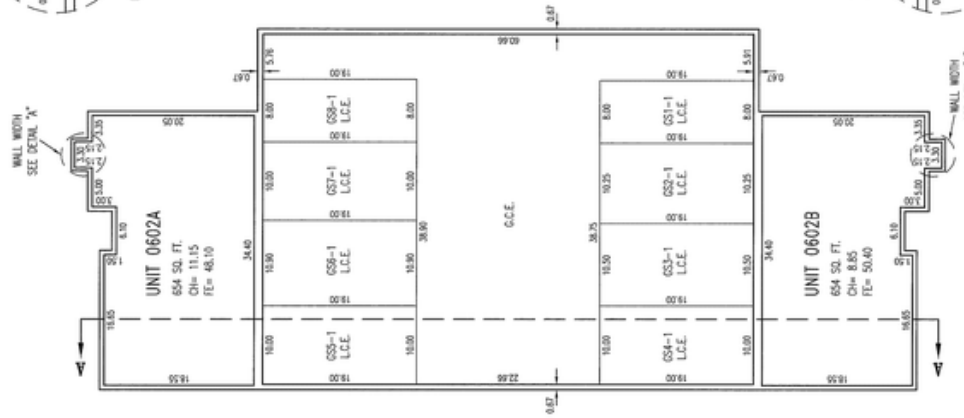
DETAIL "B" DETAIL SCALE: 1" = 5"
