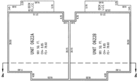
BUILDING 6 SECOND LEVEL INTERIOR WALLS 0.67" WIDE EXTERIOR WALLS 0.55" WIDE
