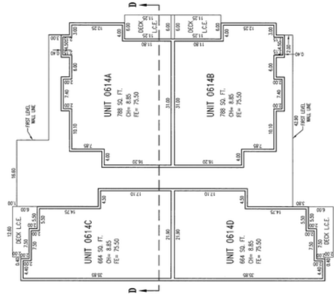
BUILDING 4 SECOND LEVEL INTERIOR WALLS 0.67" WIDE EXTERIOR WALLS 0.57" WIDE, OR AS NOTED
