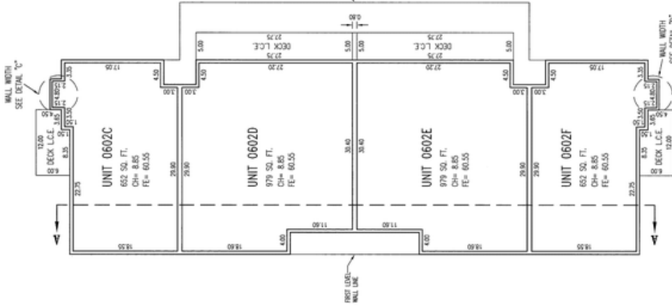
DETAIL "B" DETAIL SCALE: 1" = 5"
