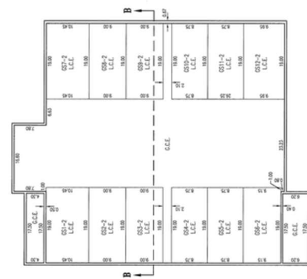
BUILDING 2 FIRST LEVEL INTERIOR WALLS 0.50" WIDE, OR AS NOTED EXTERIOR WALLS 0.50" WIDE, OR AS NOTED
